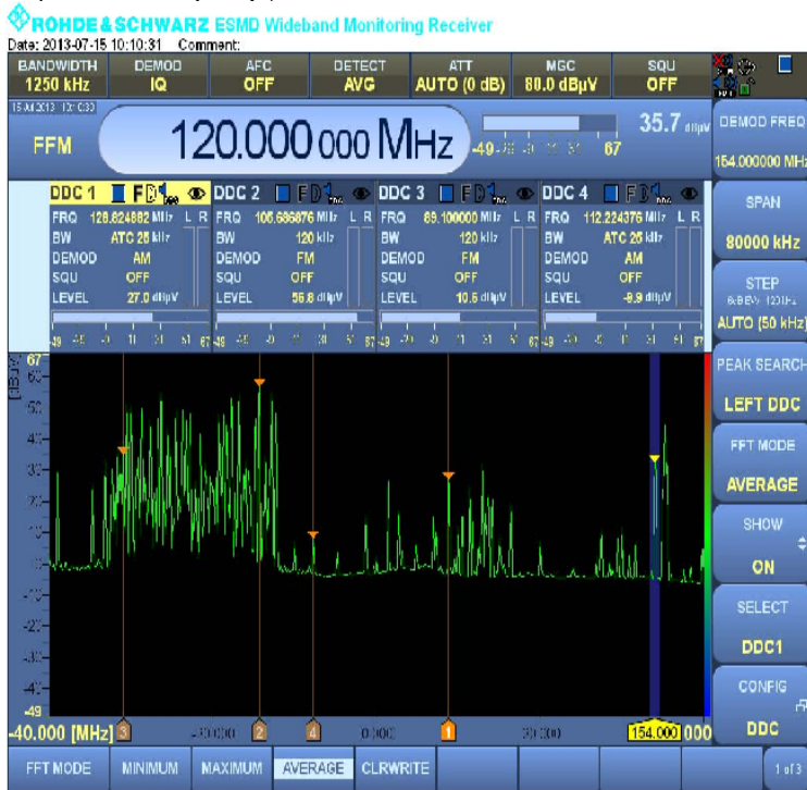
Fig 3 Five channel arrangement for signal analysis Conclusion
